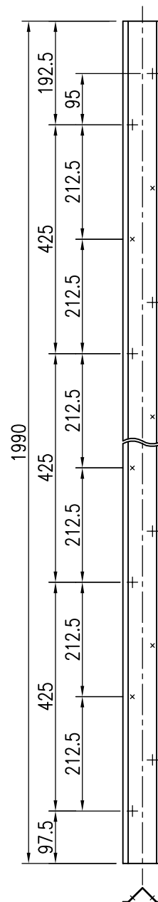
(定尺2m)
